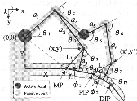
Fig.2 Device model
