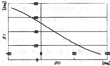
Fig. 4 Relation between \theta_1 and \theta_{f1}
