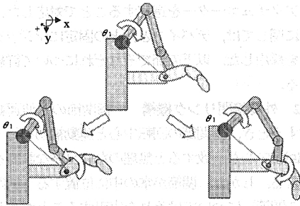
Fig. 3 Singular configuration
