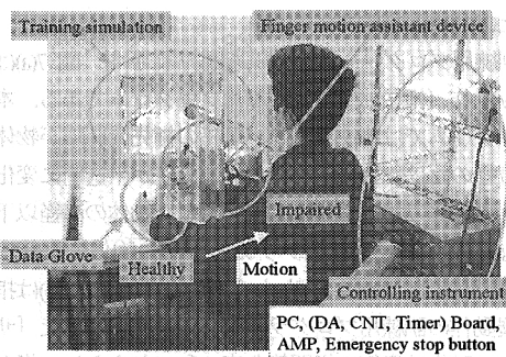
Fig.8 Overview of the system
