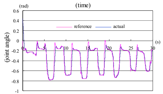
Fig.8. Result of the self-motion control experiment
