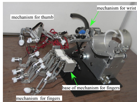
Fig. 1 photo of the motion assistance equipment
