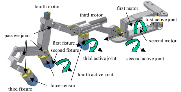
(b) Mechanism for thumb
