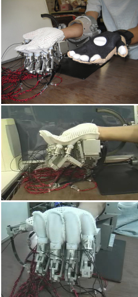
Fig.7. Snapshot of the Self-motion control experiment
