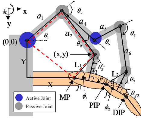
Fig. 3. Closed loop structure composed of the mechanism and finger
