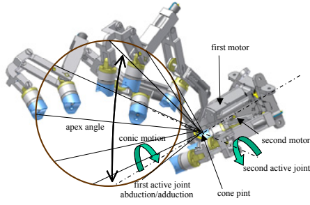
Fig. 4. Conic motion-assisting CM joint
