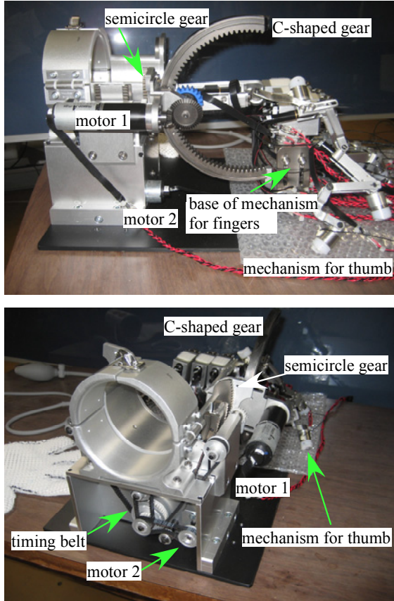
Fig. 5. Motion assistance mechanism for the wrist
