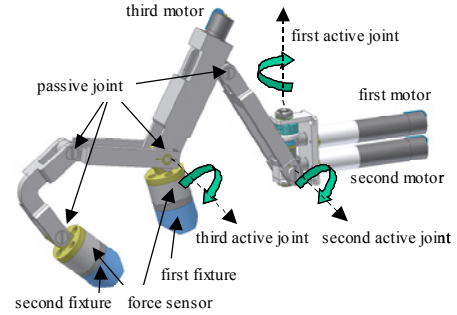
(a) Mechanism for fingers
